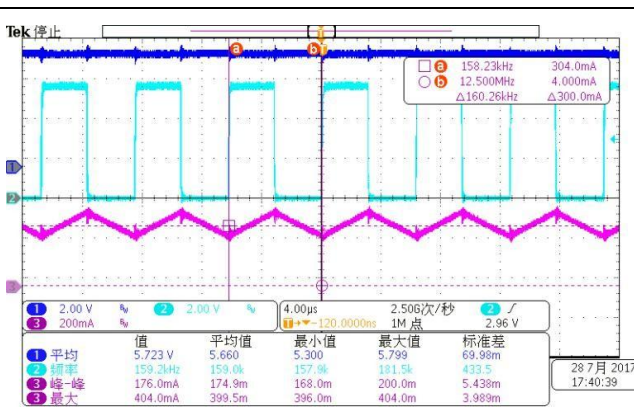
图2: 48Vin/8LEDs (CH1:VDD CH2:V GATE CH3:I out )
