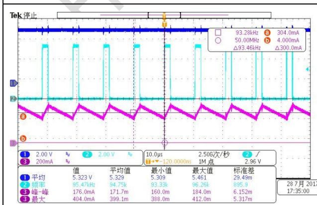
图1: 48Vin/3LEDs (CH1:VDD CH2:V GATE CH3:I out )
